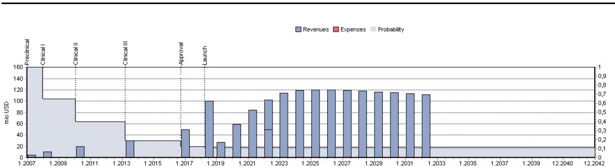
Figure 1: Cash flow Adnexus Therapeutics with USD 2,000 Mio sales.
